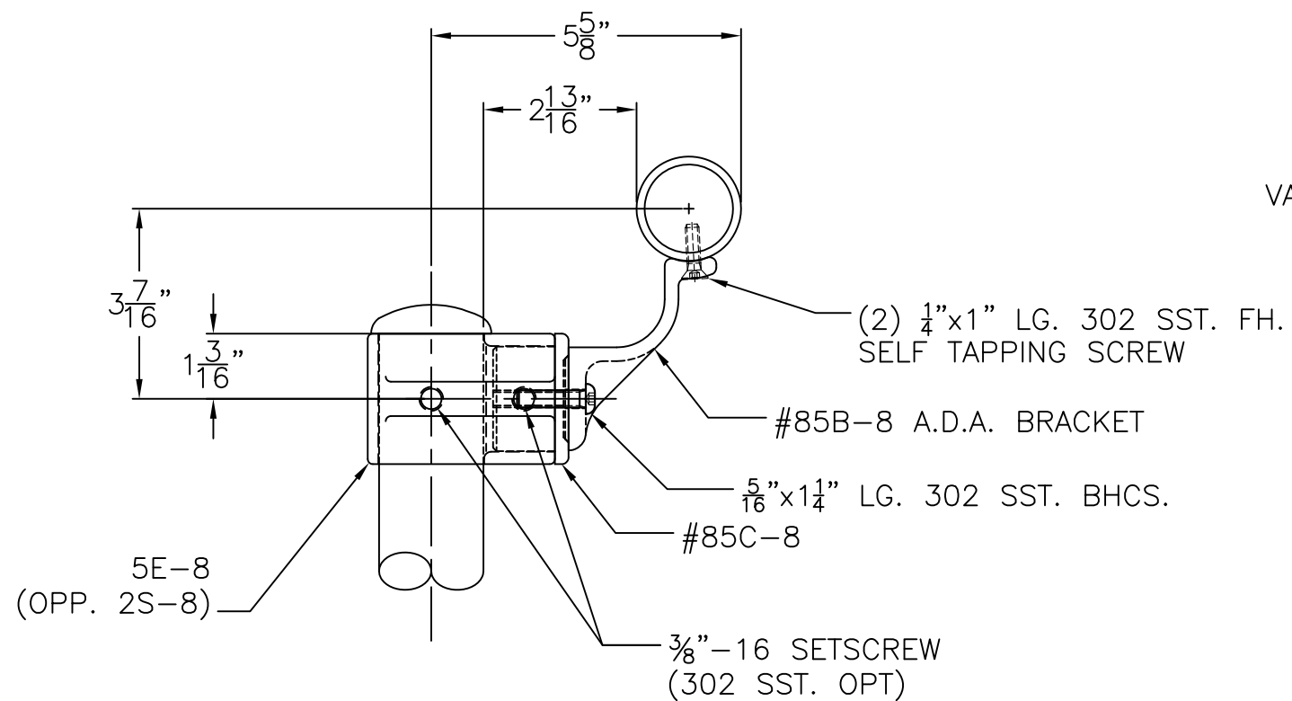
#285 SPEED RAIL. BRACKET POST MOUNTING (VARI-SLOPE)
