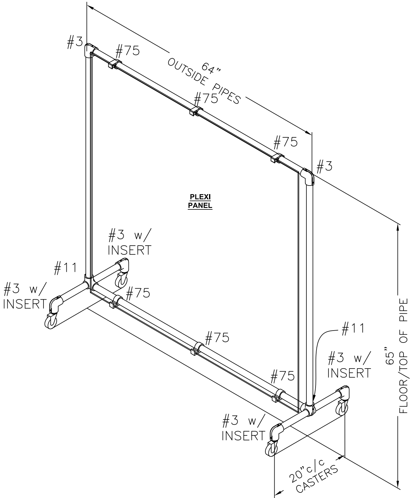
Speed Rail ® Safety Shield - Rack "A" Offset 64" L. x 65" H
